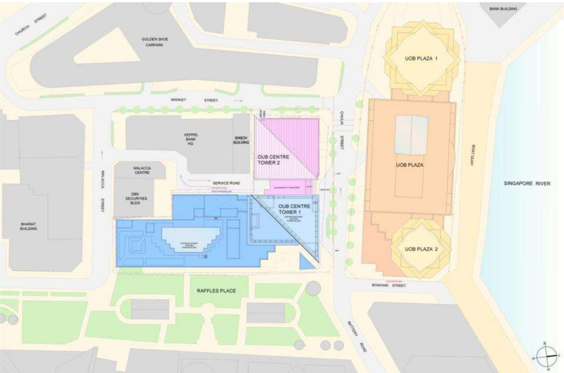
SITE PLAN
